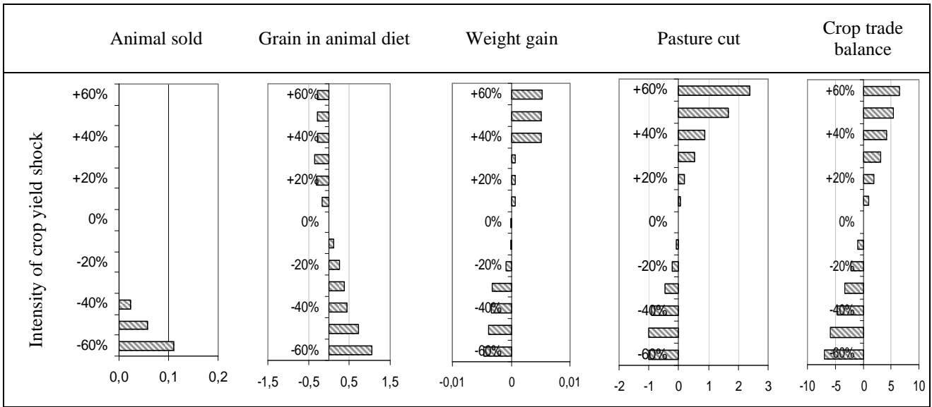
Figure 1: Rate of variation of production management indicators between year of shock occurrence (n3) and equilibrium level according to shock intensity (a: beef price shock, b: crop yield shock.)
